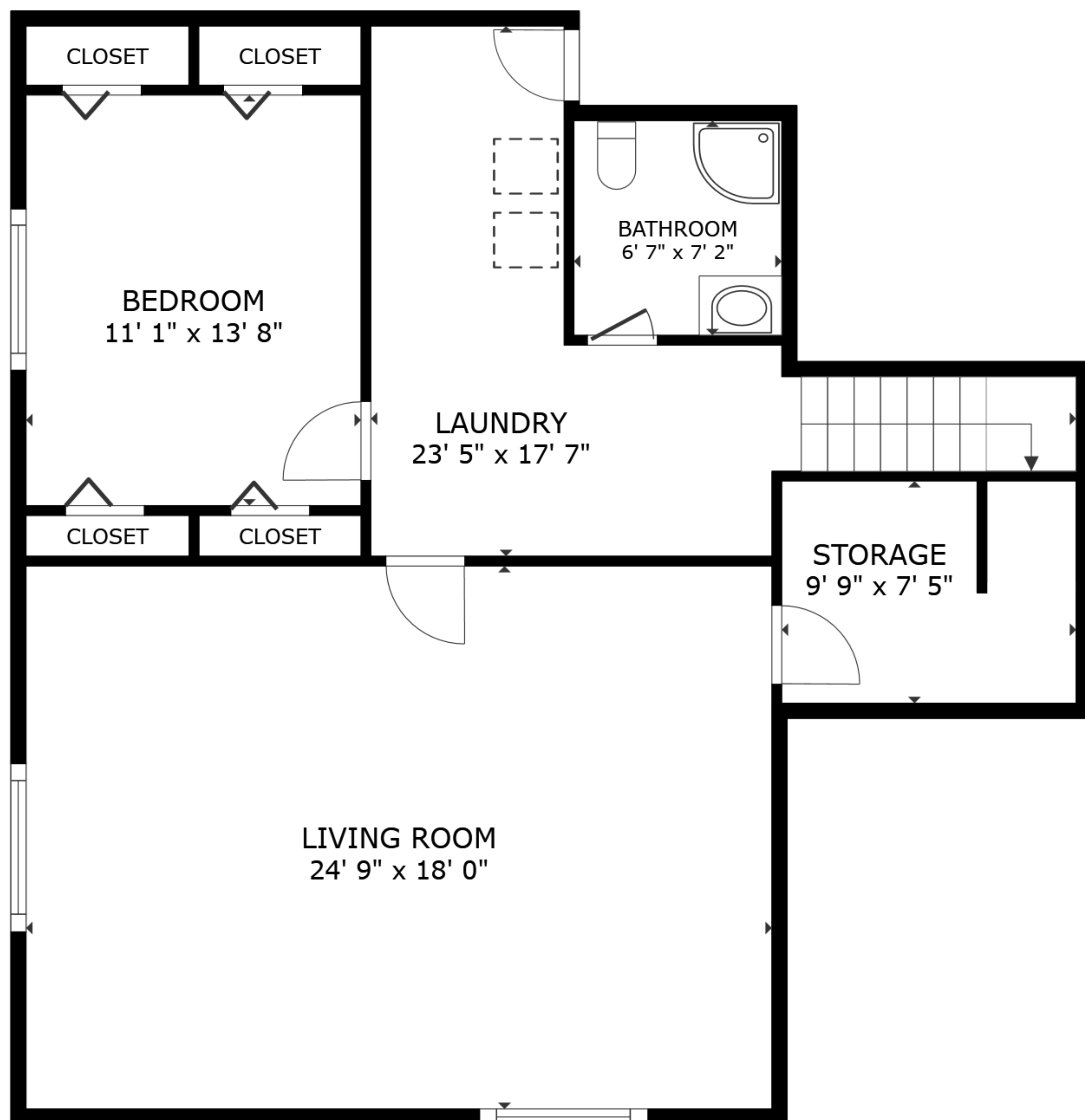
FLOOR 1
