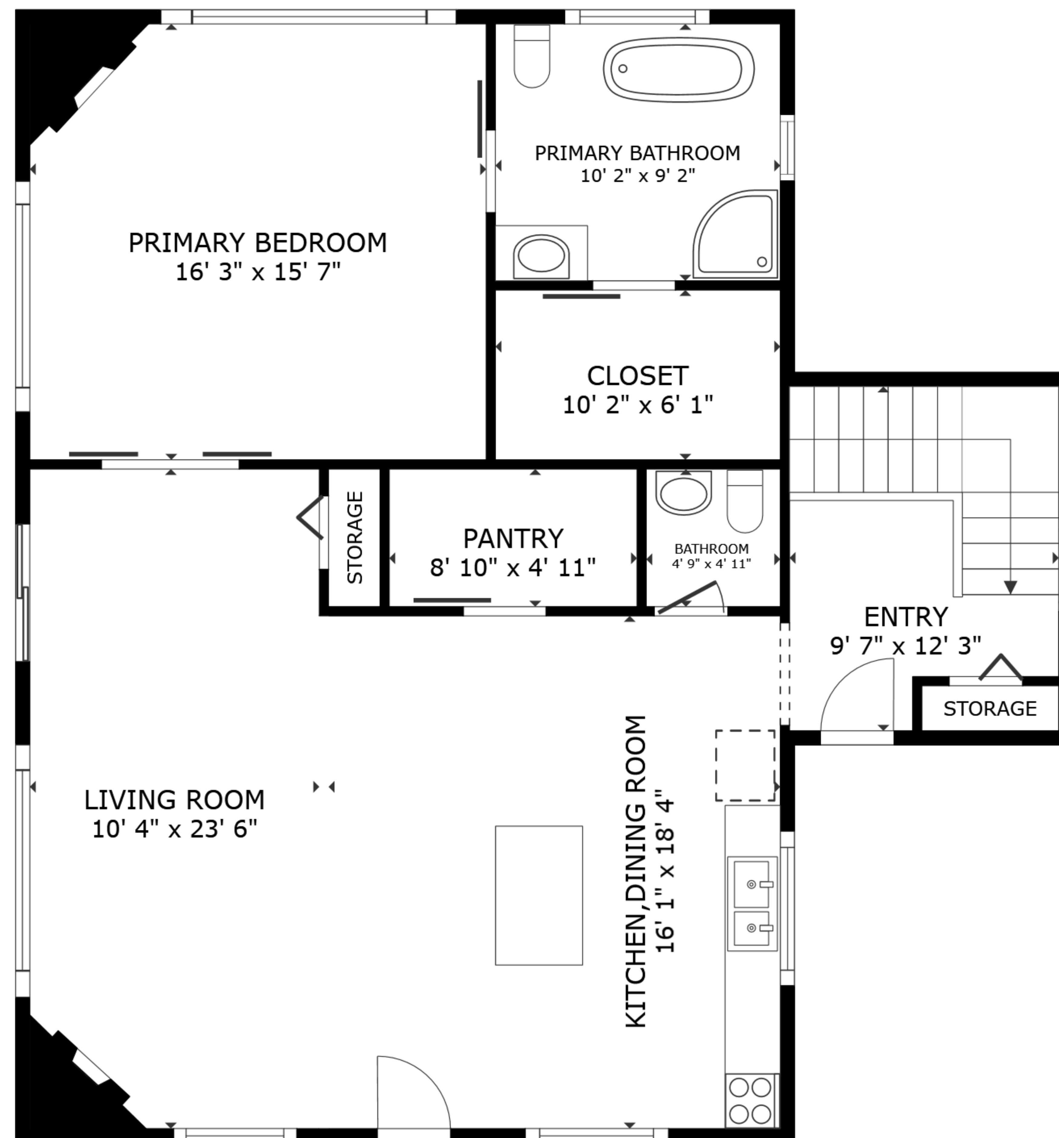
FLOOR 2
