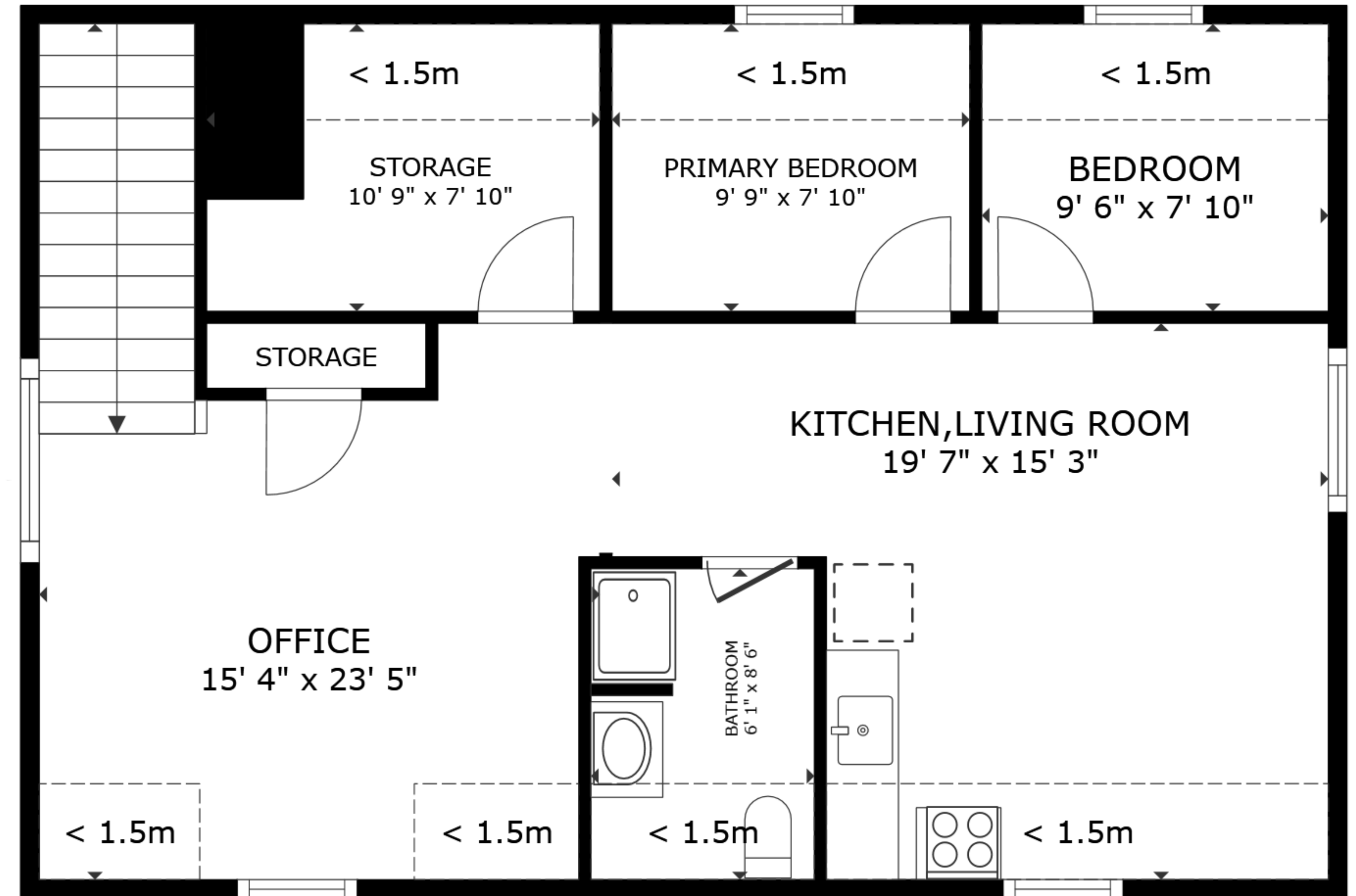
FLOOR 2
